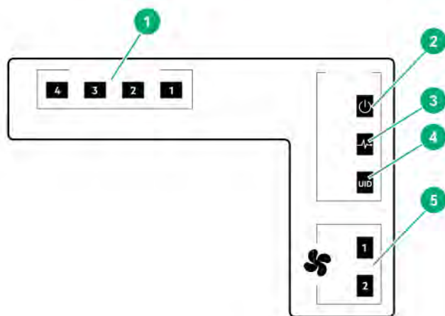
Figure 2: Rear panel LEDs for 6400 switch series
