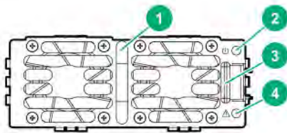
Figure 6: Aruba X382 54DC 2700W AC Power Supply (JL372A)
